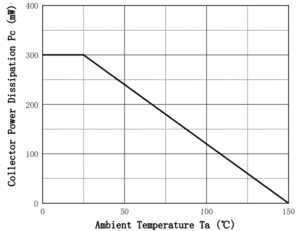
Fig. 8 - Collector Power Derating Curve
