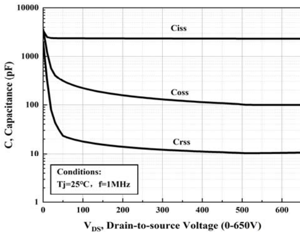
Figure 13. Capacitances vs. Drain Source Voltage (0-650V)
