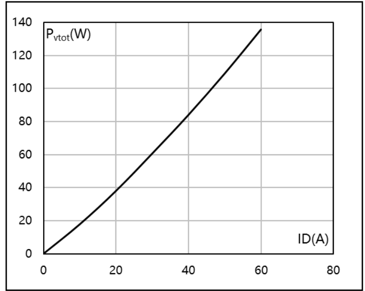
Fig2. Power dissipation
