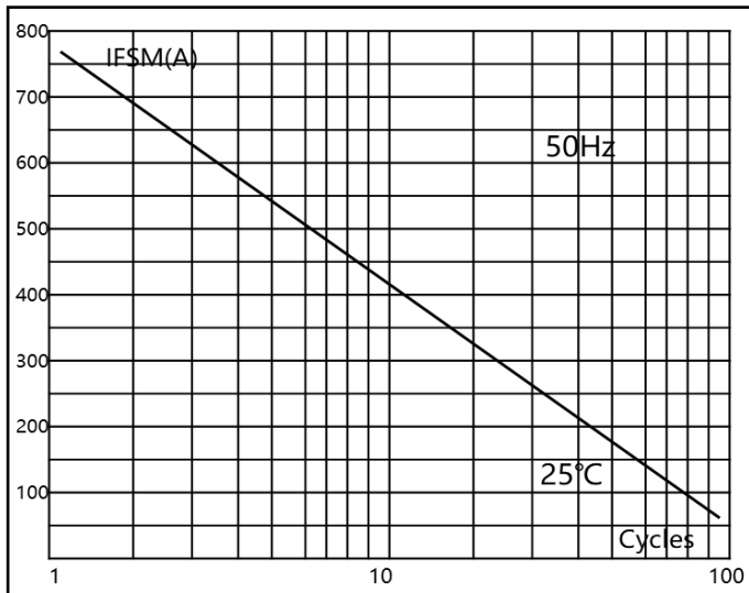
Fig3. Max Non-Repetitive Forward Surge Current
